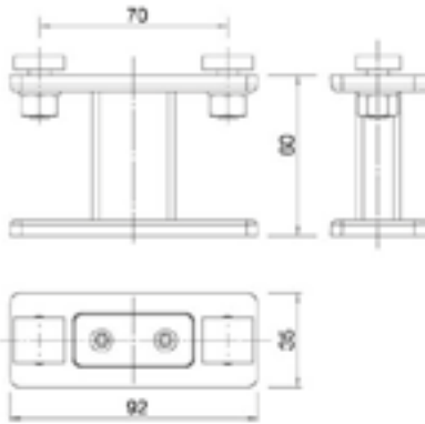
B-Winkel PS-601-1 Standard
