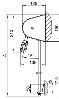
Wandmontage
